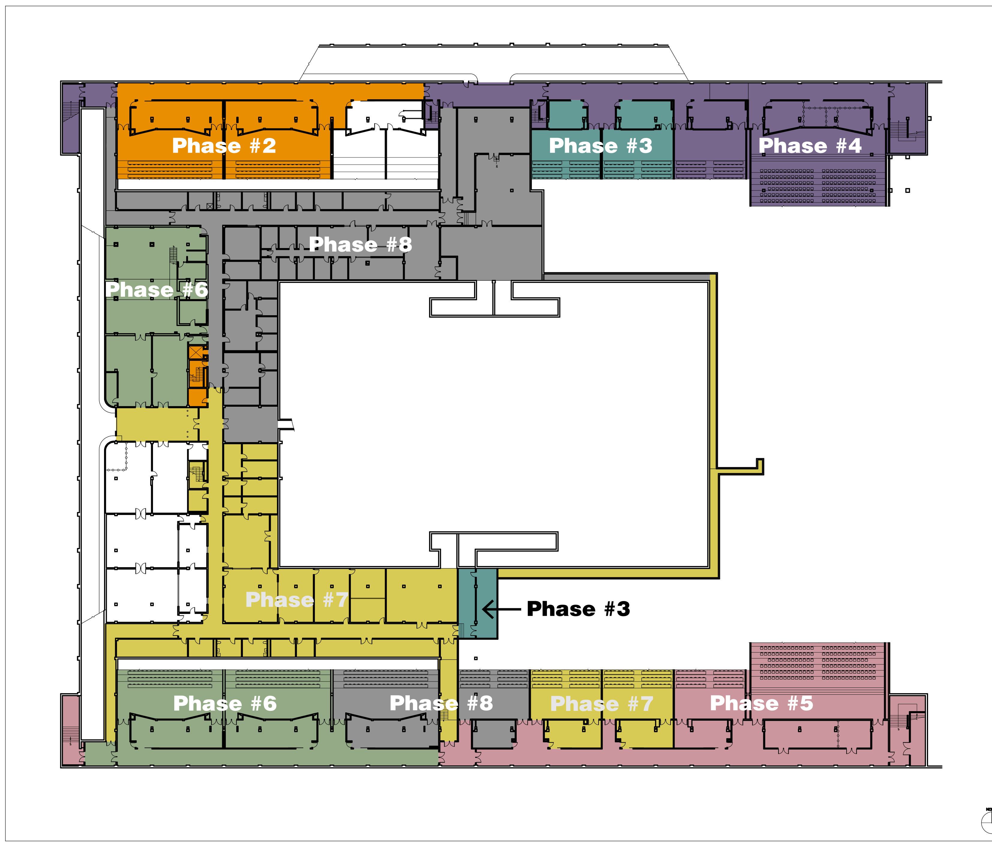
SUB BASEMENT PHASING PLAN SCALE: 1/32" = 1'-0"
