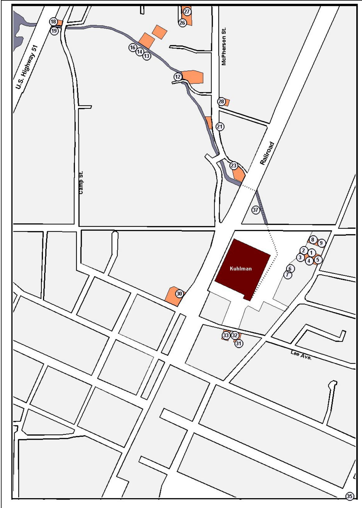
Map of Tree Bark sampling "CS-" sites (Hermanson, 2003).
