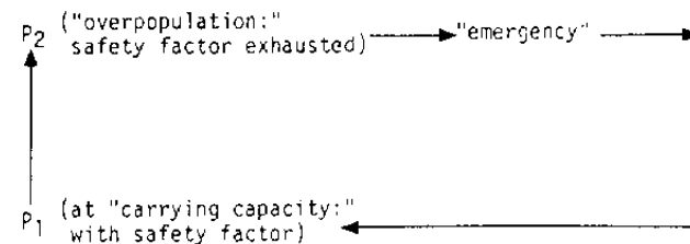
Figure 13.1 The population cycle of a nation that has no effective, conscious population control, and which receives no aid from the outside. P_2 is greater than P_1 .
