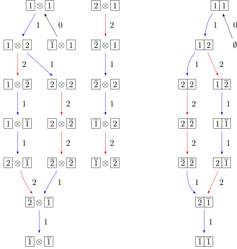
FIGURE 1. The crystals \tilde{D}_1(B^{1,1} \otimes B^{1,1}) (left) and \tilde{D}_1(B^{1,2}) (right) in Example 4.4.
