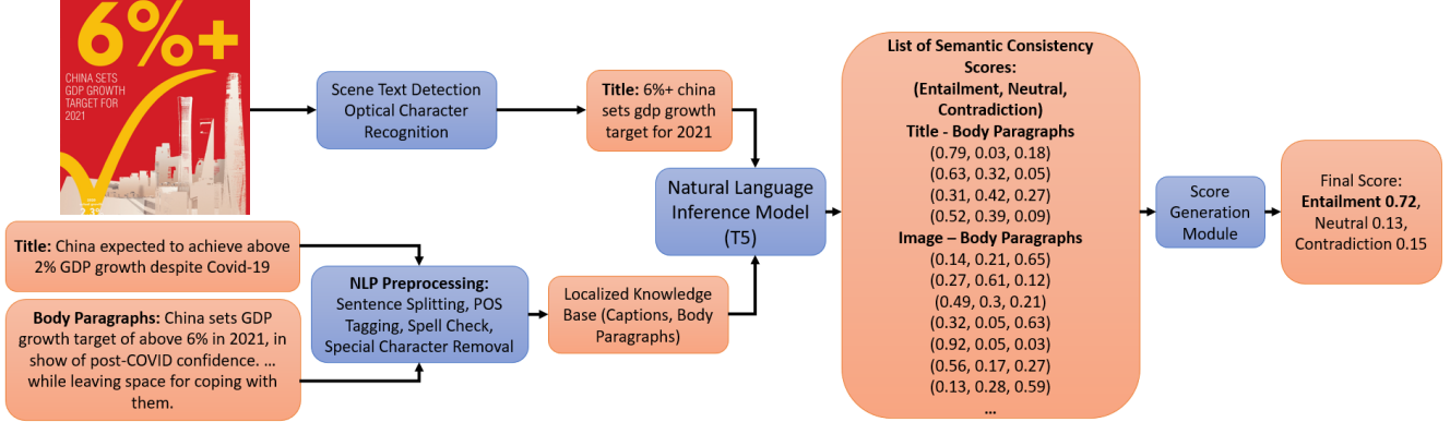
Figure 2: An example showing the proposed infographic consistency analysis pipeline. Infographic images are processed by the scene text extractor. Titles and body paragraphs are then pre-processed into a knowledge base. The T5 inference model is then used to verify all textual claim pairs based on the structure of the input according to Table 1. All inference scores are then normalized and condensed using the score generation module to create a final semantic consistency score for the whole article.
