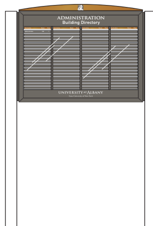
LB-3-Modified-A Directory: 4 column Scale: 3/8"=1'-0" Page 3:4
