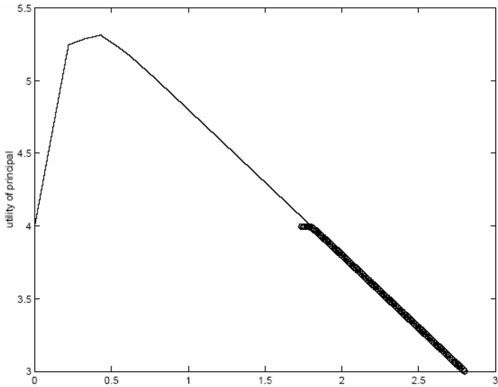
Figure 2: Example 3. “ooo”: Semi-RP value function; “---”: full-commitment value function
