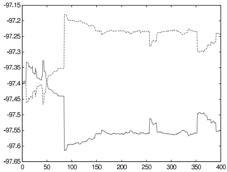
Figure 3: Sample path 2. Upper panel: effort paths. Lower panel: expected utility paths. ‘-.-’ = agent 1; ‘—’ = agent 2.
