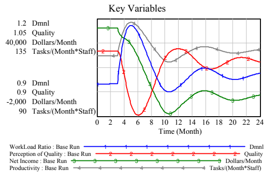
Figure 21—Base Run
