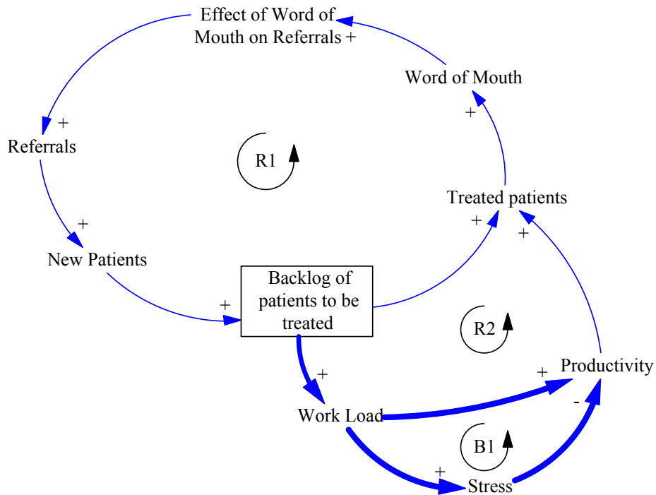
Figure 9—Productivity Loop
