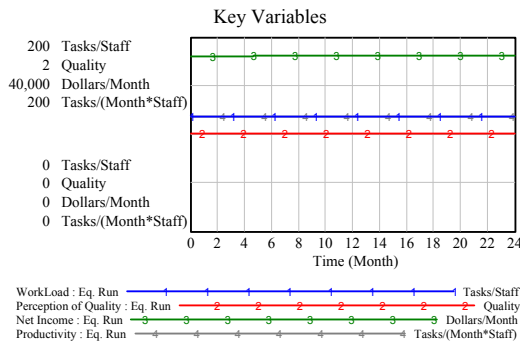
Figure 20—Equilibrium Run
