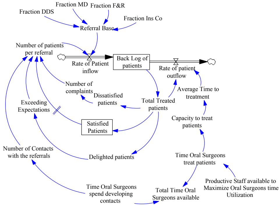
Figure 19—Satisfaction Structure
