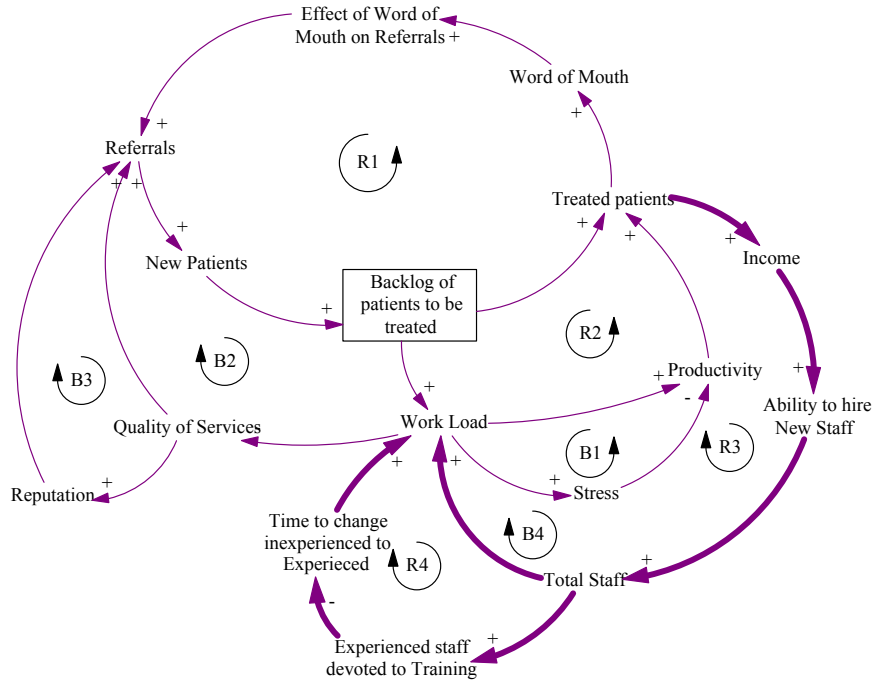
Figure 12—Productivity/Staff Loop
