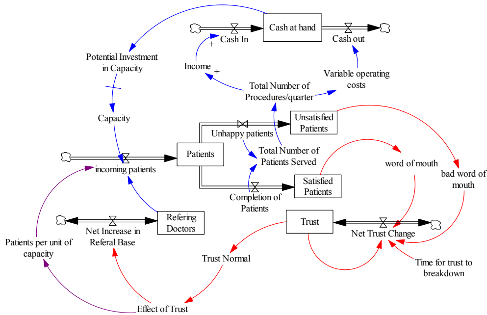
Figure 16—Concept Model
