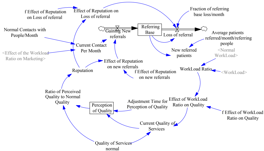
Figure 18—Referring-Base Structure
