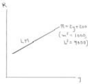
Figure 1: LM Curve
